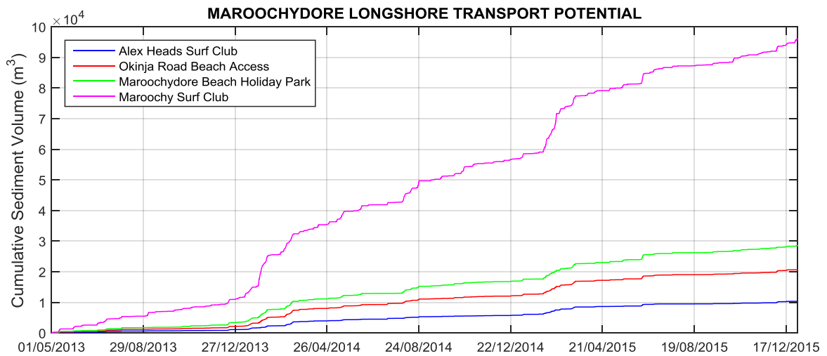
Figure 4-9 Cumulative Volume of Longshore Sediment Transport
