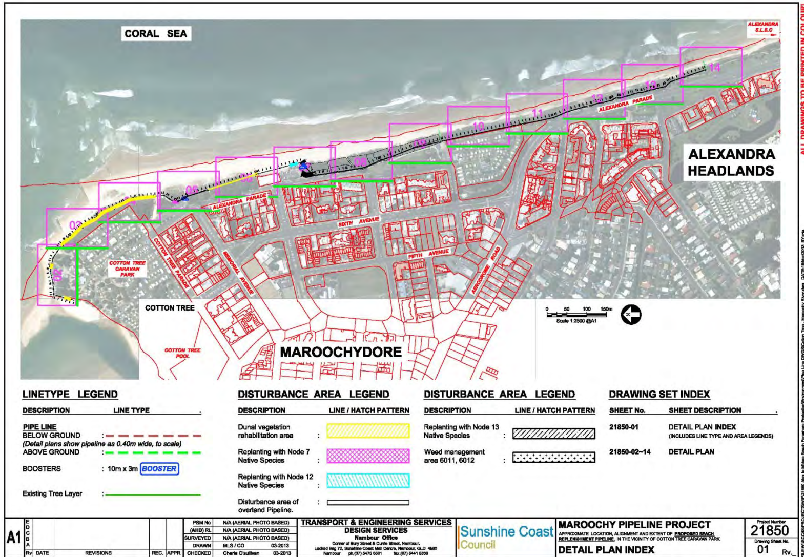
Figure 3-1 Slurry Pipeline Alignment and Disturbance Areas
