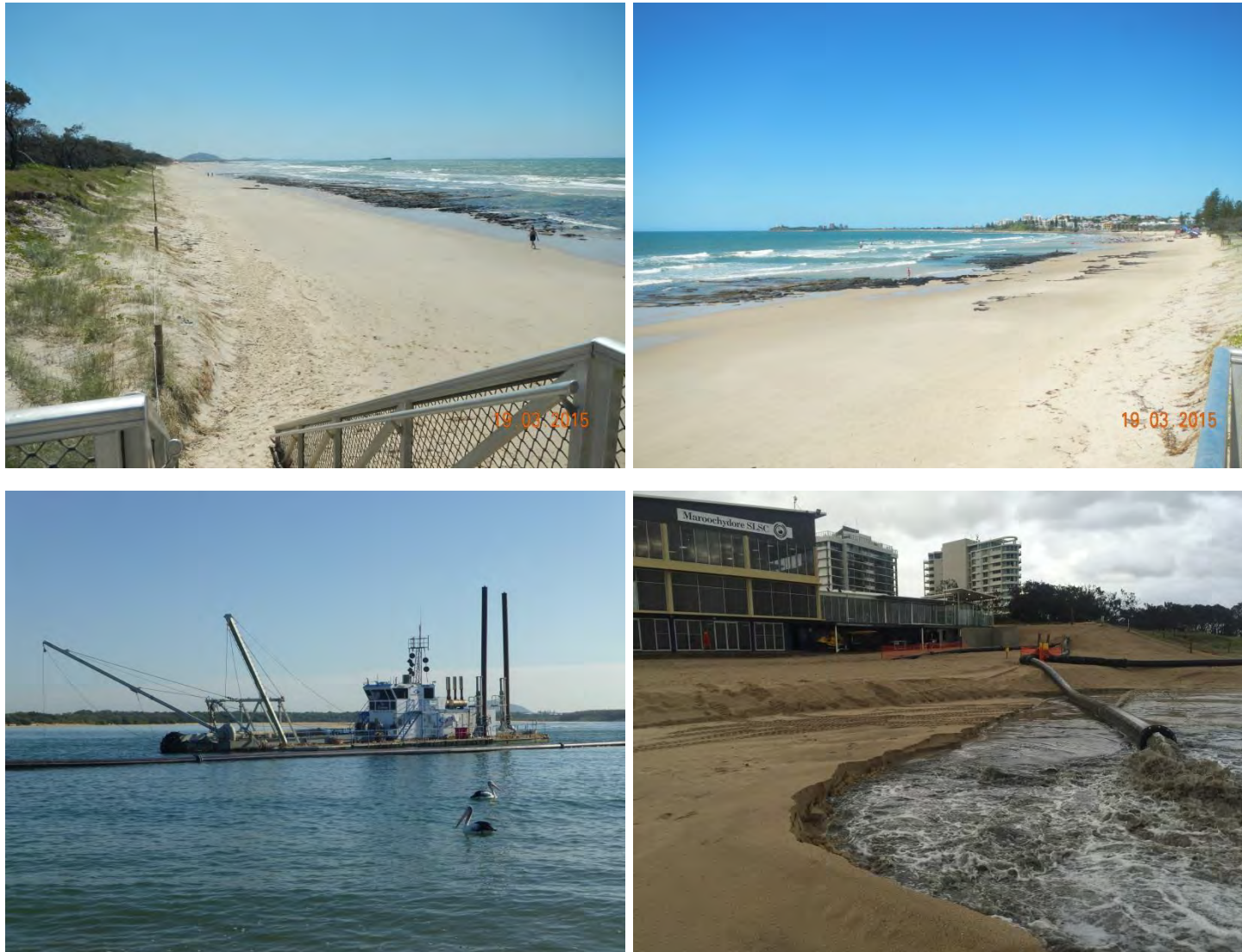
Figure 3-3 Stage 2 Dredging and Nourishment (clockwise from top left): Pre-works Beach Condition North; Pre-works Beach Condition South; Pipeline Sand Delivery to Maroochydore Beach; Neumann CSD Nu Endeavour in the Lower Maroochy River
