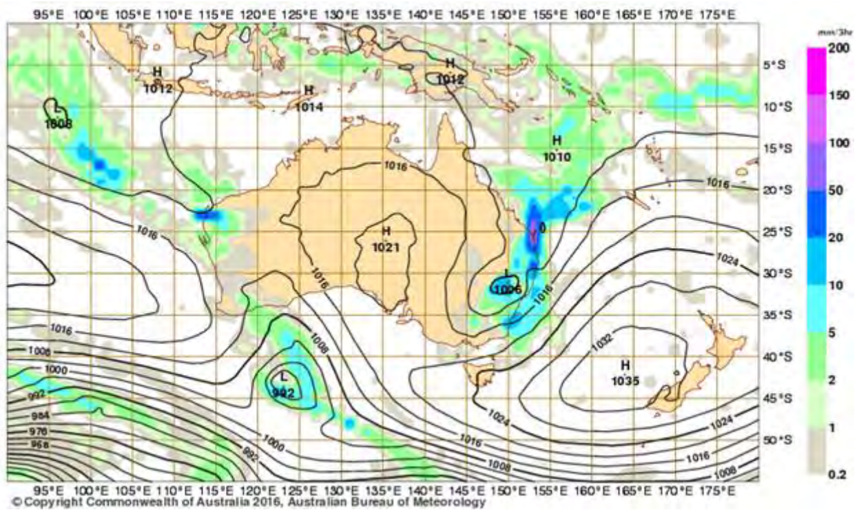
Figure 4-2 June 2016 East Coast Low – Mean Sea Level Pressure and Precipitation Composite Map
