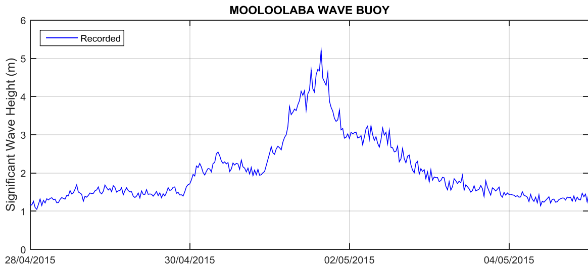
Figure 4-8 Recordings at the Mooloolaba Wave Buoy during the April/May 2015 ECL (data provided by DSITI)
